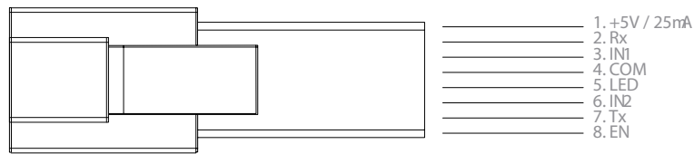
Fig.4: SPI terminals
