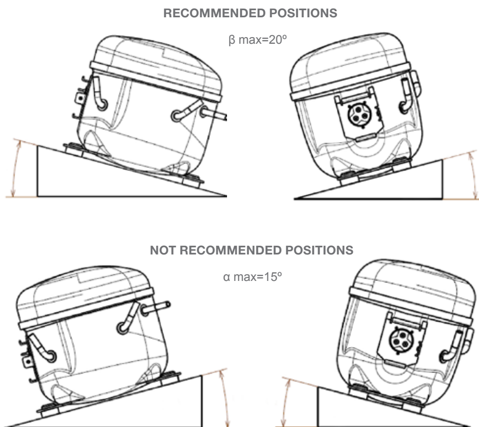
Fig.1: Maximum tilt angle
