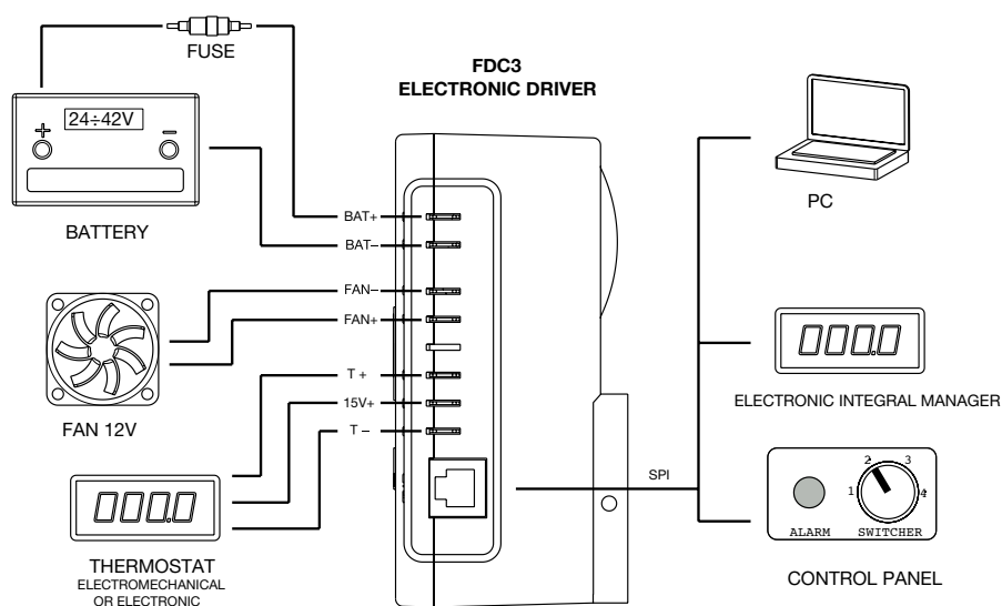
Fig.2: FDC3 wiring scheme
