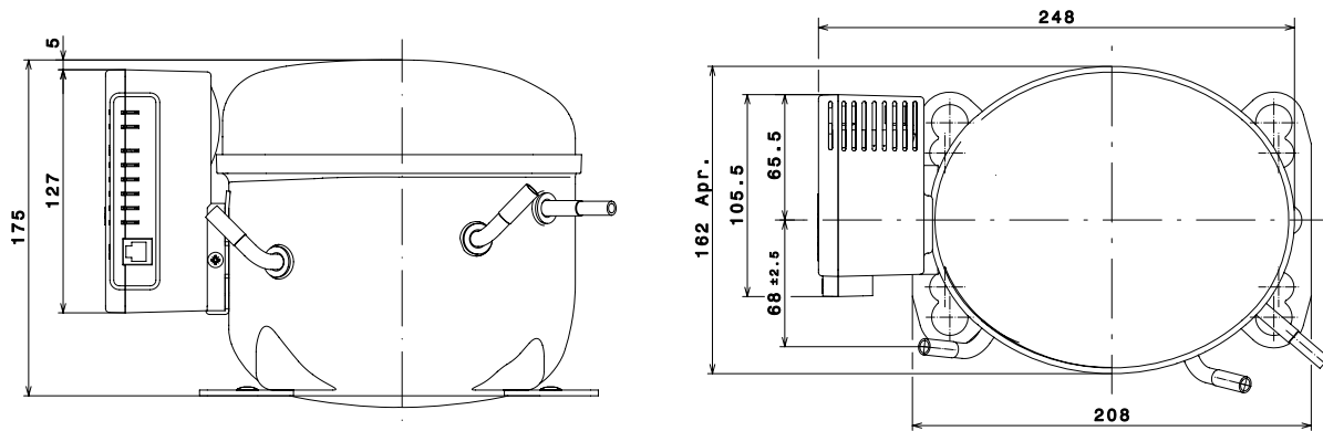
Fig.5: GLT80TDC outline drawing
